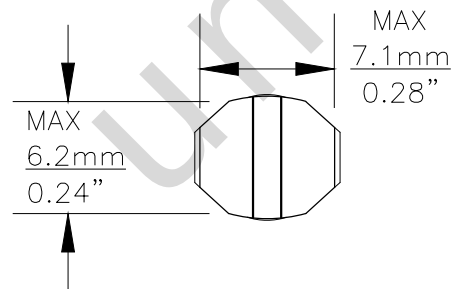
BASE BOTTOM VIEW
